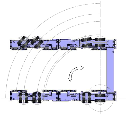
Front-wheels steering
