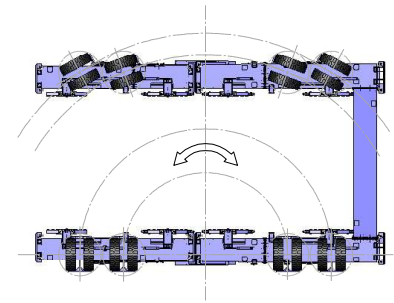
Concentric steering
