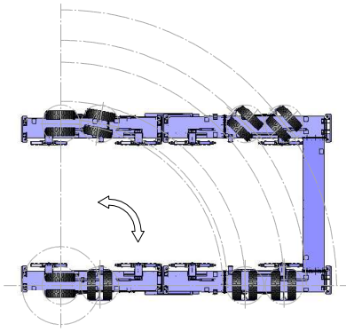
Rear-wheels steering
